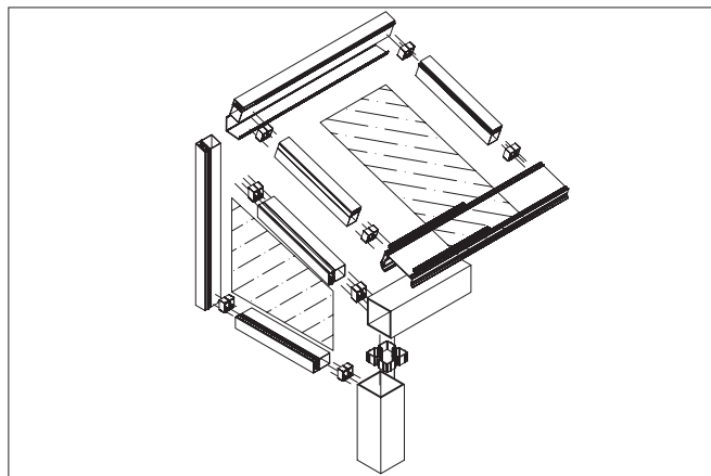
Lasikattorakenne
